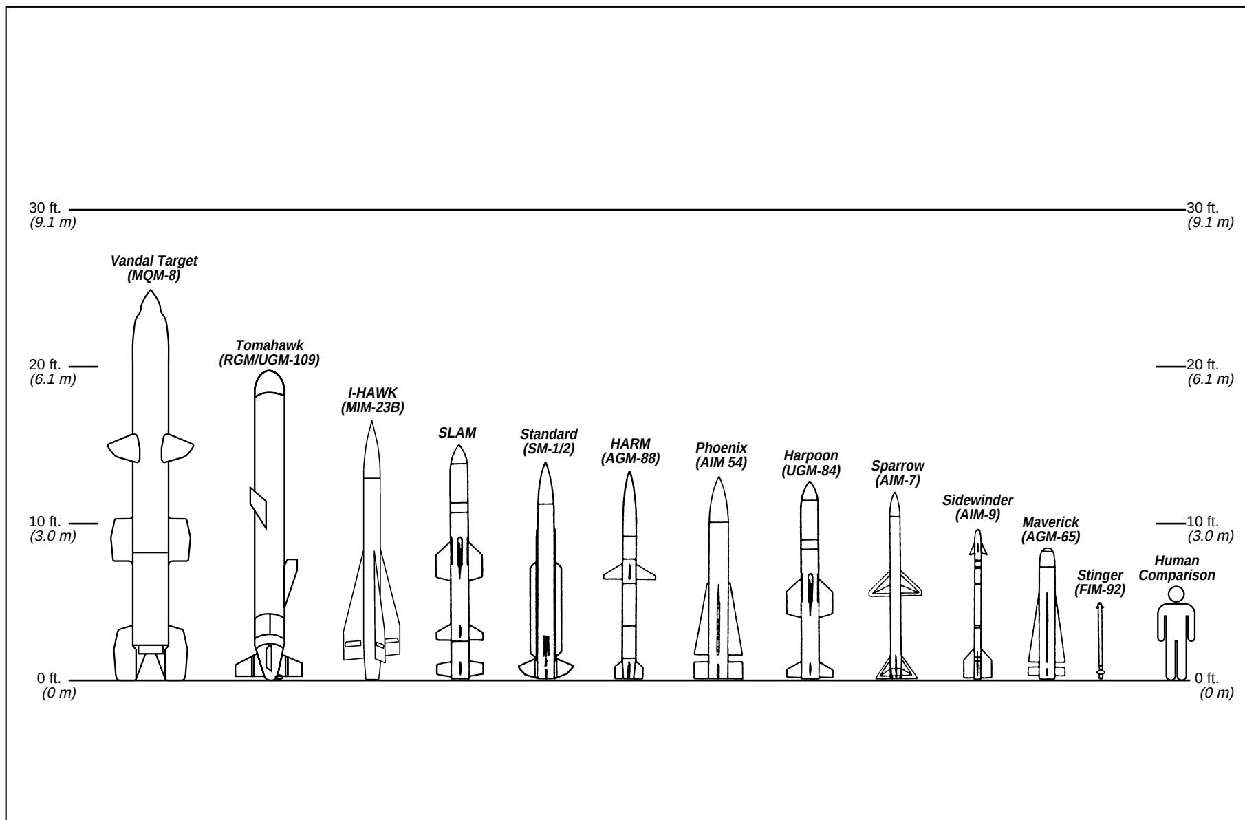
Figure 3.0-10 Typical Missiles Used at Point Mugu Sea Range
