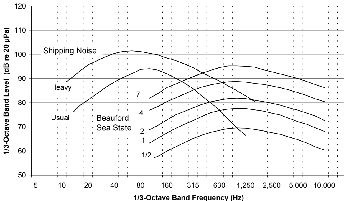
Figure D-8 Underwater Ambient Noise
