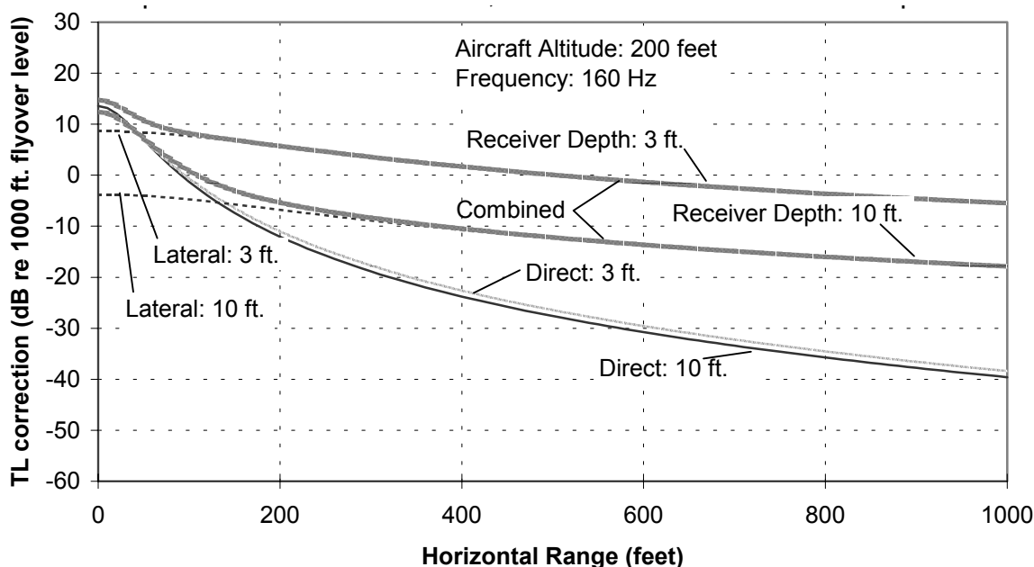
Figure D-6 Transmission Loss of Noise through Air-Water Interface, Comparison of Direct-Refracted, Lateral and Combined TL Components
