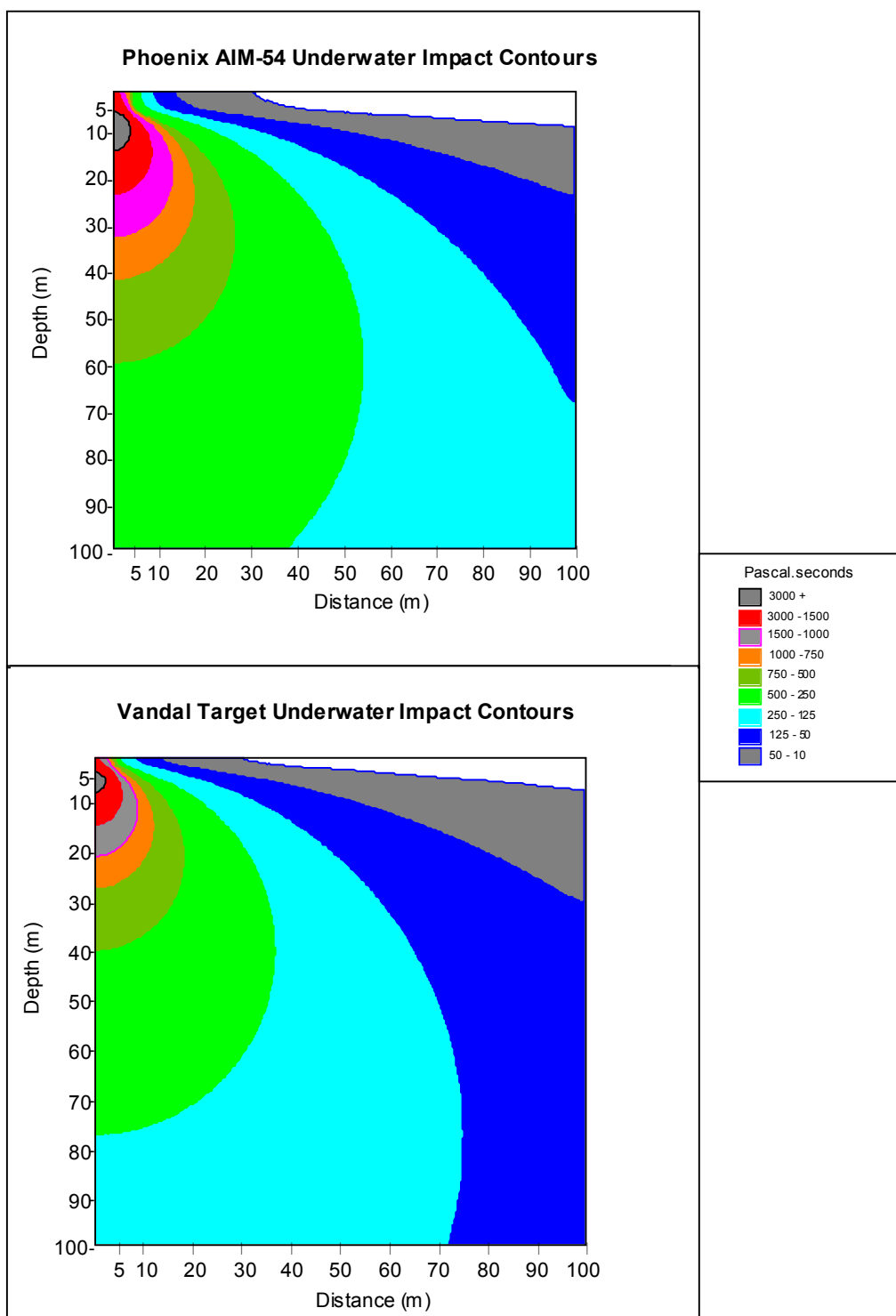
Figure 4.7-4 Underwater Impact Contours in Pascal.seconds for an Intact Phoenix Missile and Vandal Target Hitting the Water. Calculated as described in the text and the Marine Mammal Technical Report .
