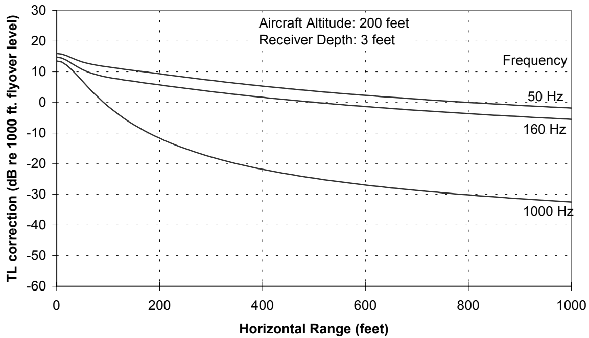
Figure D-7A Air-Water Transmission Loss vs. Frequency
