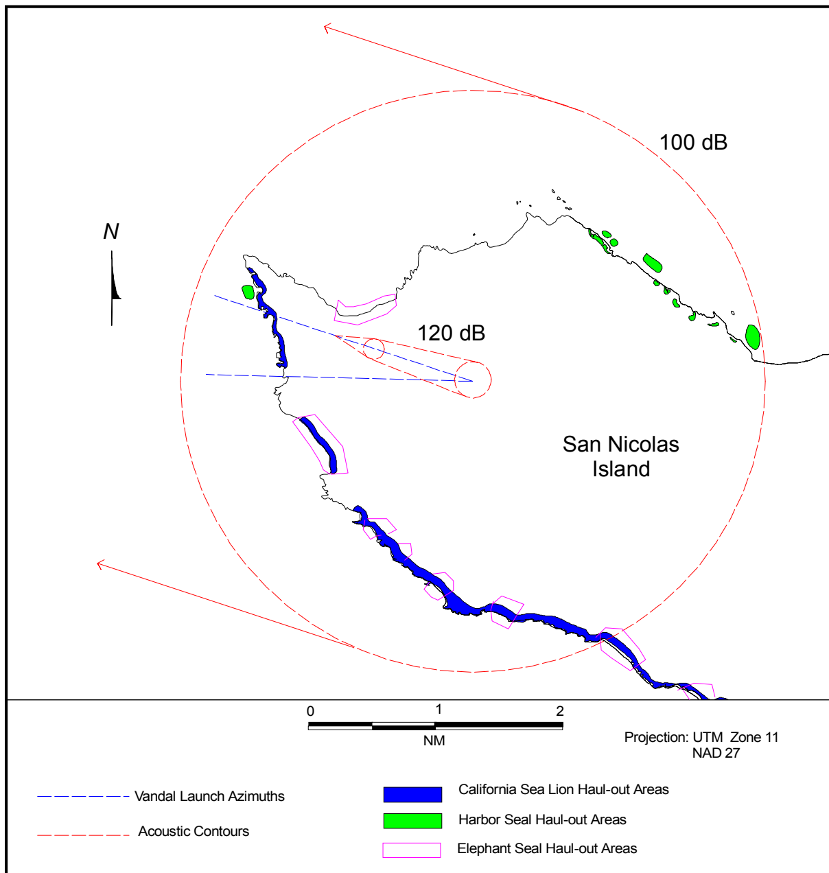
Figure 4.7-3 The 100 and 120 dB re 20 \mu Pa Acoustic Contours for Vandal Target Launches from San Nicolas Island on an A-weighted Sound Exposure Level (SEL) Basis.
