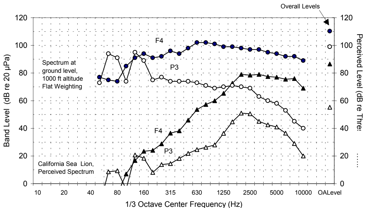
Figure D-3 Aircraft Noise Spectra vs. Hearing Response
