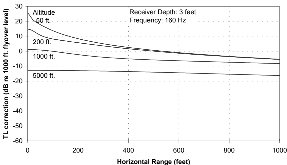
Figure D-7C Air-Water Transmission Loss vs. Aircraft Altitude
