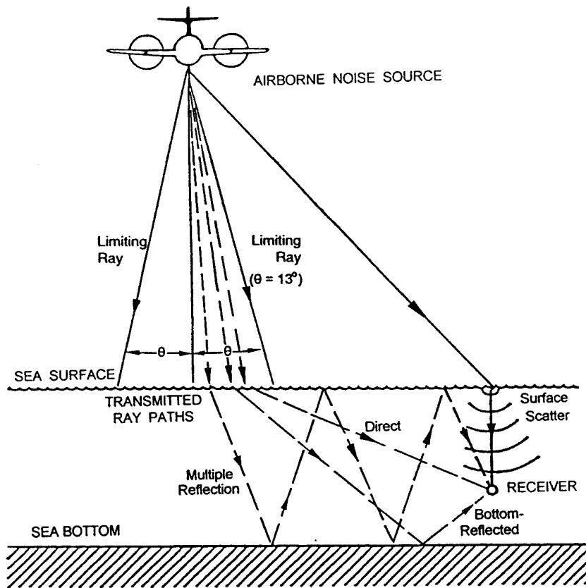
Figure D-5 Characteristics of Sound Transmission through Air-Water Interface
