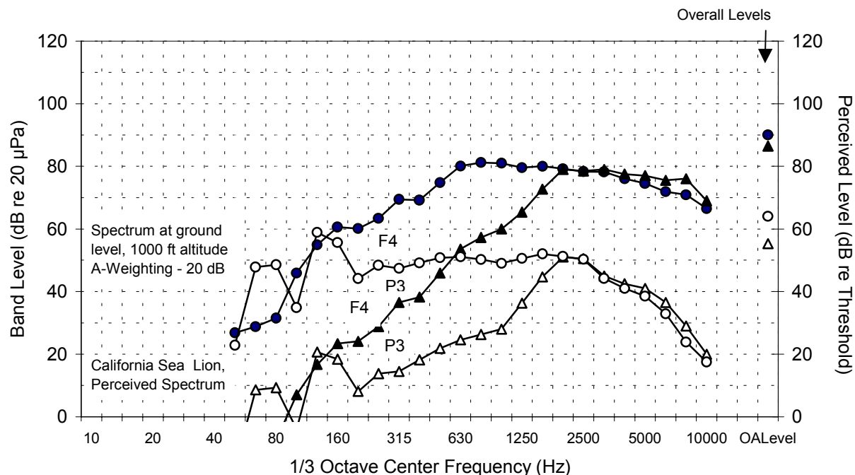
Figure D-4 Adjusted A-Weighting of Aircraft Noise vs. Hearing Response
