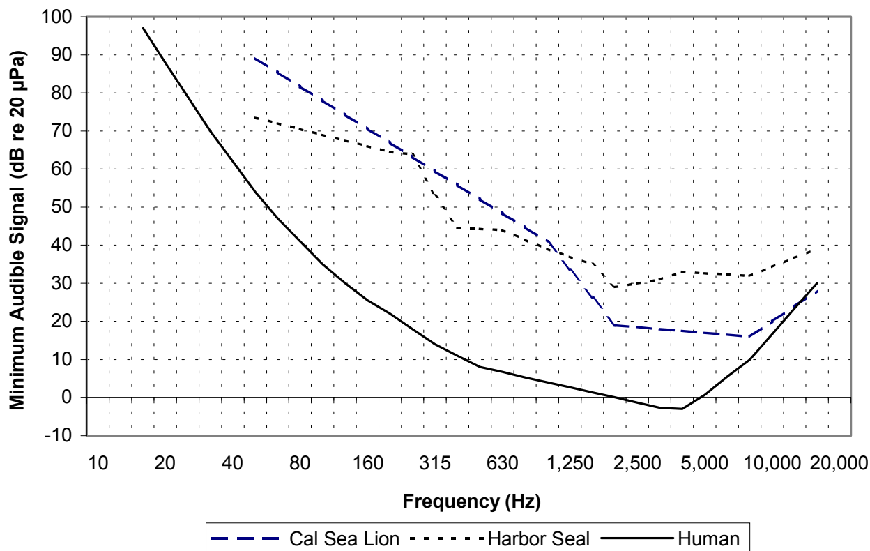
Figure D-1 Human and Marine Mammal In-Air Hearing Thresholds
