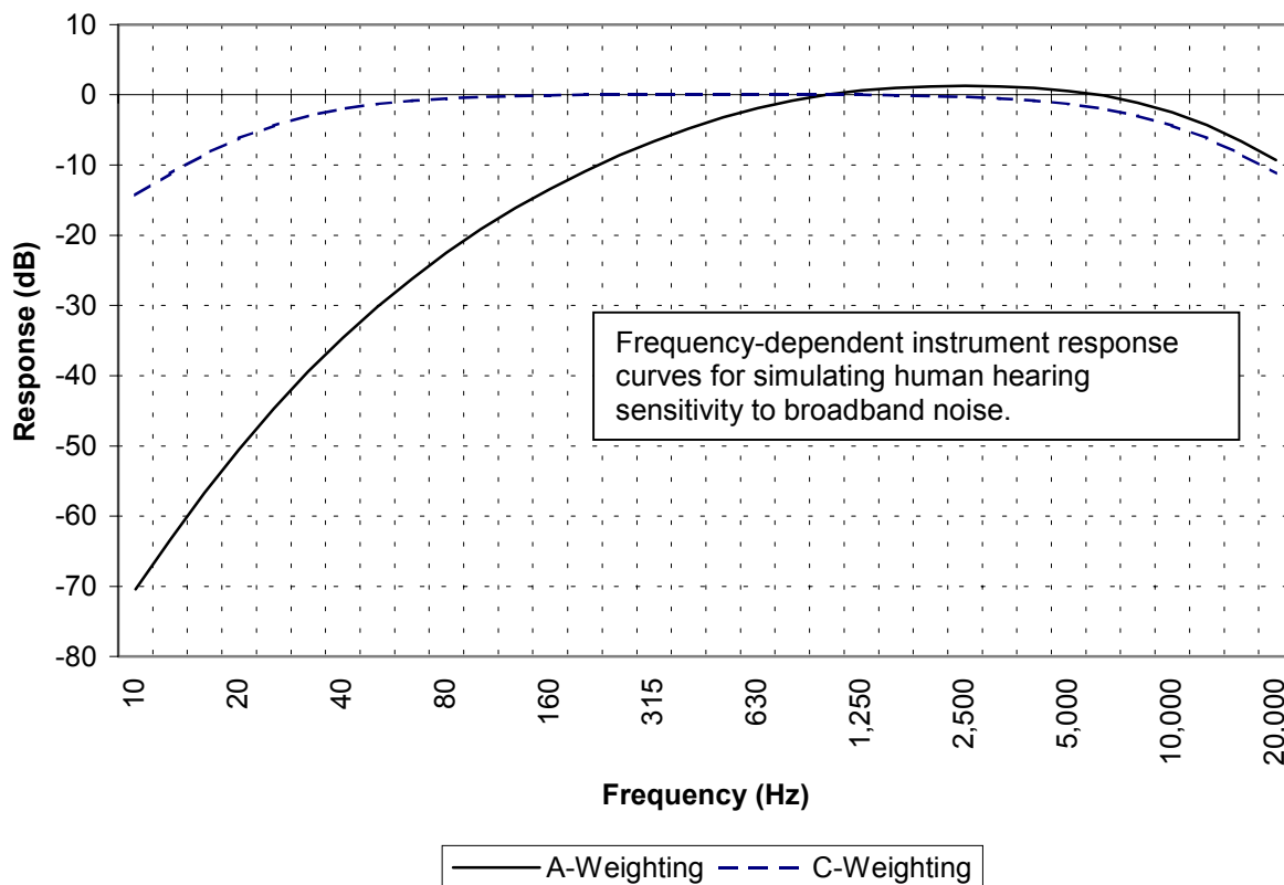
Figure D-2 Noise Weighting Characteristics
