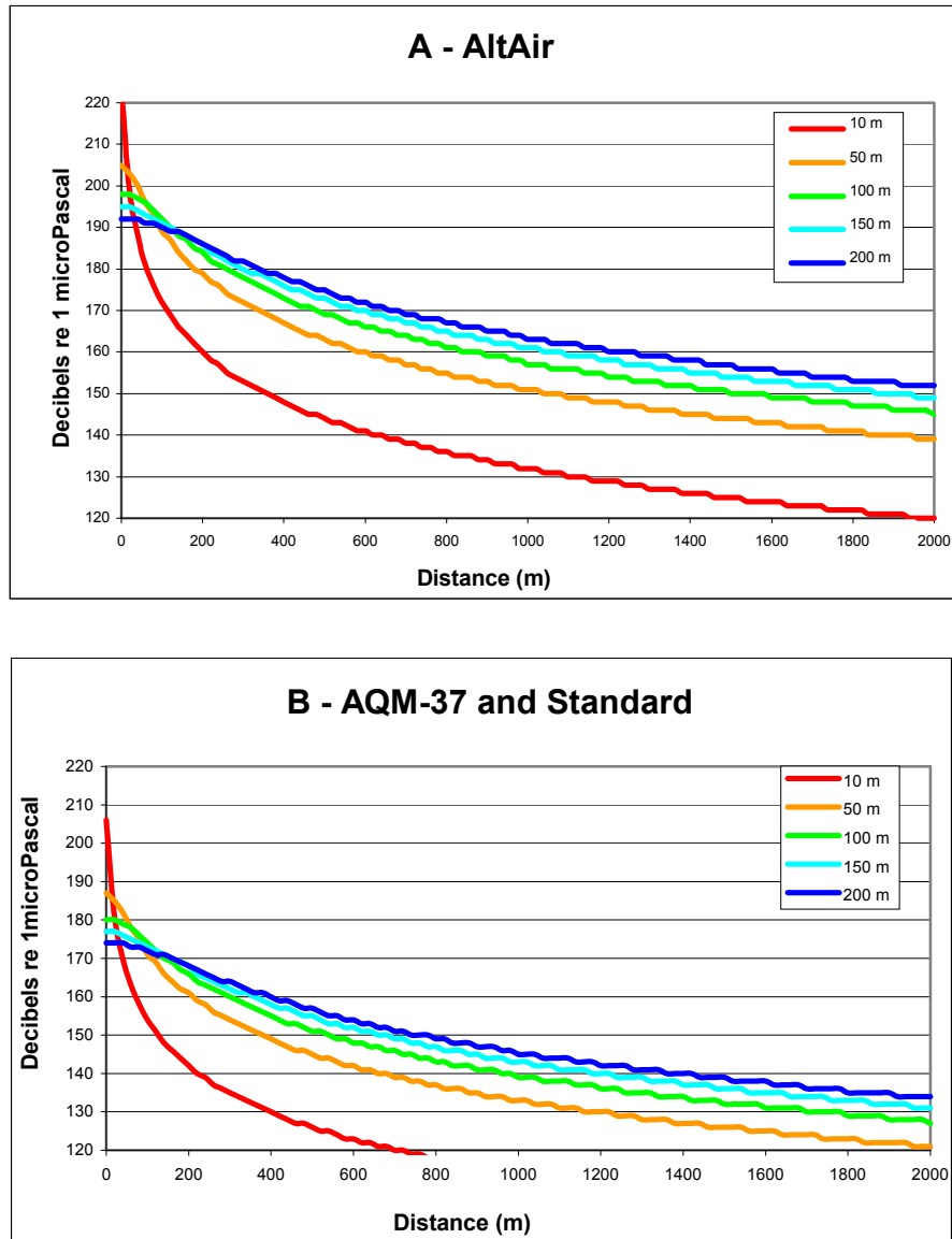
Figure 4.7-6 Sound Pressure Levels at Five Depths for Various Intact Missiles, Targets, and Mines Hitting the Water.
