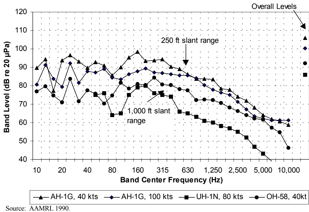
Figure D-9C Noise Spectra: Helicopters
