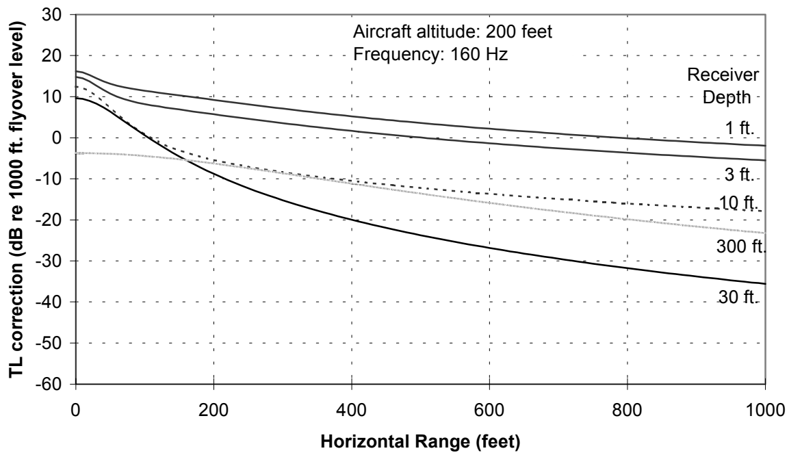
Figure D-7B Air-Water Transmission Loss vs. Receiver Depth
