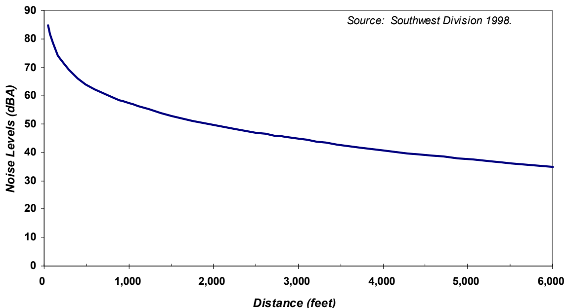
Figure 4.3-1 Typical CNELs Associated with Construction Activity (in dBA)
