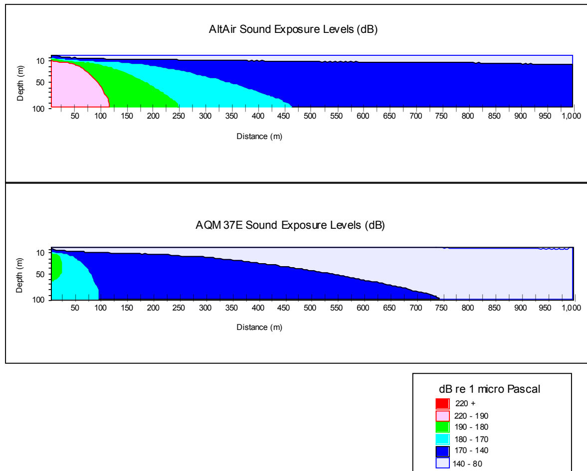
Figure 4.7-5 Sound Pressure Level Contours for Intact AltAir and AQM-37/Sidewinder Missiles Hitting the Water.
