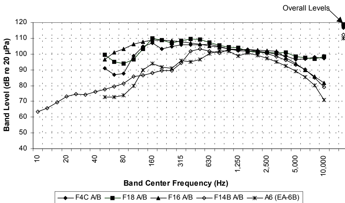
Figure D-9A Noise Spectra: Fighter and Attack Aircraft
