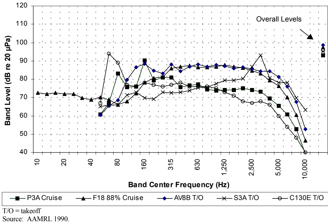
Figure D-9B Noise Spectra: Selected Sea Range Aircraft
